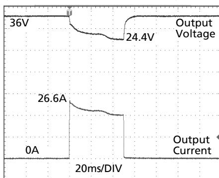
Fig. 27-3 Peak load 26.6A for 50ms, typ.
