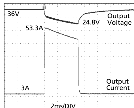
Fig. 27-4 Peak load 53.3A for 5ms, typ.
