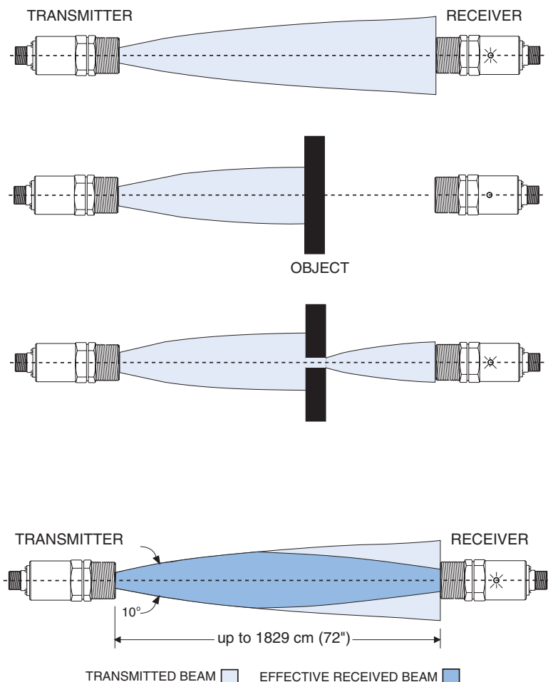
Figure 1, Thru-beam Pattern and Range
