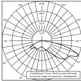
RESTL Test Report #: PL10097-001B ARE-EDG-2MP-**-06-E-UL-525-40K Initial Delivered Lumens: 9,149
