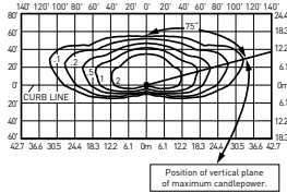
ARE-EDG-2MB-**-10-E-UL-525-40K Mounting Height: 25' (7.6m) A.F.G. Initial Delivered Lumens: 13,185 Initial FC at grade
