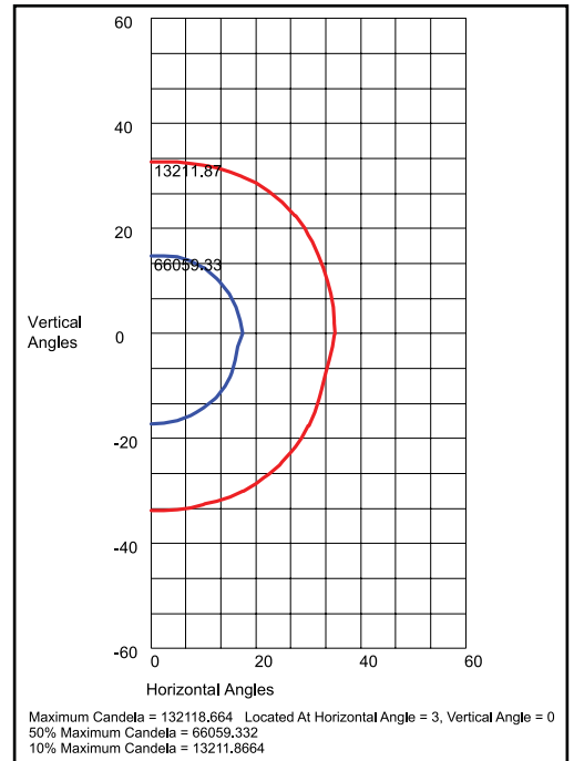
KH55QI2X256U5KC* 30°H x 30°V, NEMA 4H x 4V
