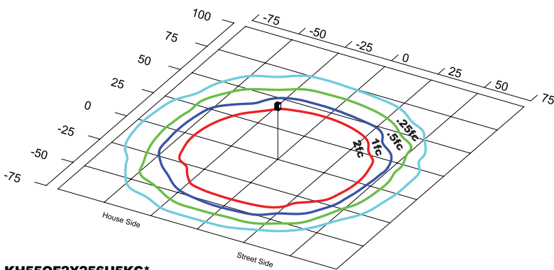
KH55QF2X256U5KC* Type V Grid in MH MH=25 Feet
