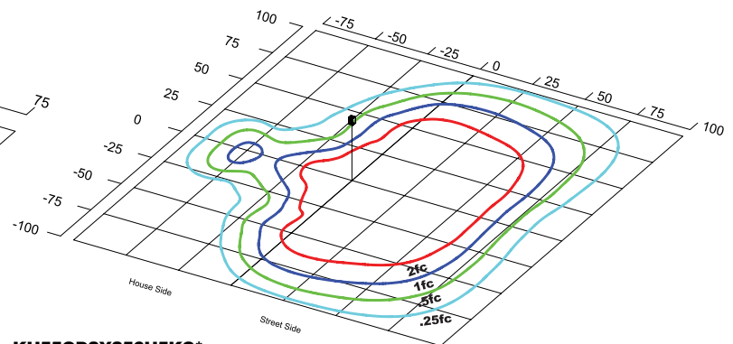
KH55QD2X256U5KC* Type IV Grid in MH MH=25 Feet
