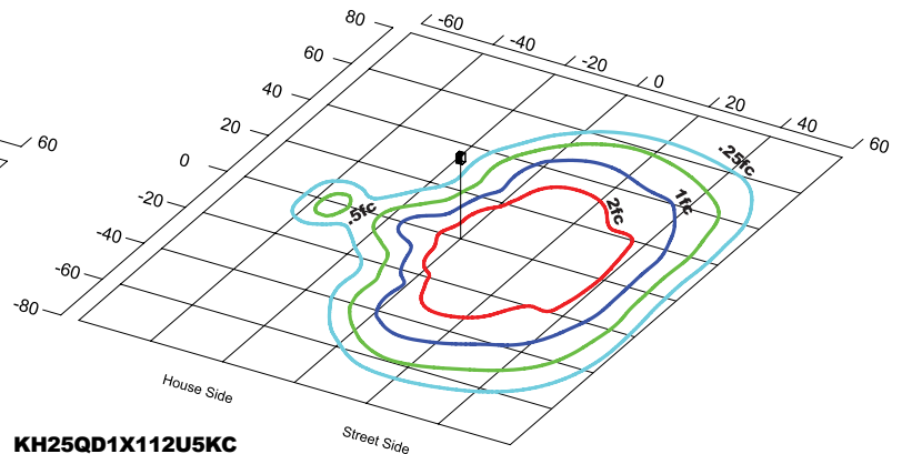
KH25QD1X112U5KC Type IV Grid in MH MH=20 Feet
