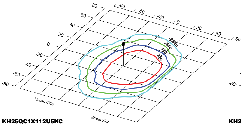
KH25QC1X112U5KC Type III Grid in MH MH=20 Feet
