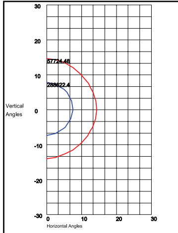
SP52Q22536U5K 19°H x 15°V Beam, NEMA 2H x 2V All values shown for 536 watt, 5K model.
