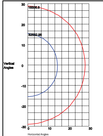
SP52Q44536U5K 31°H x 31°V Beam, NEMA 4H x 4V
