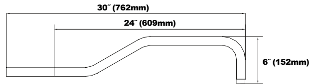
GNA03330P Straight Offset
