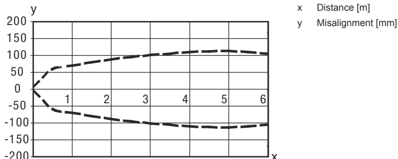
Typ. response behavior (TK 100x100)
