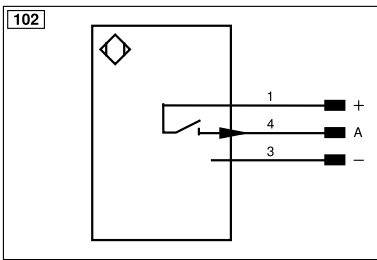
1 = Switching Status Indicator All dimensions in mm (1 mm = 0.03937 Inch)
